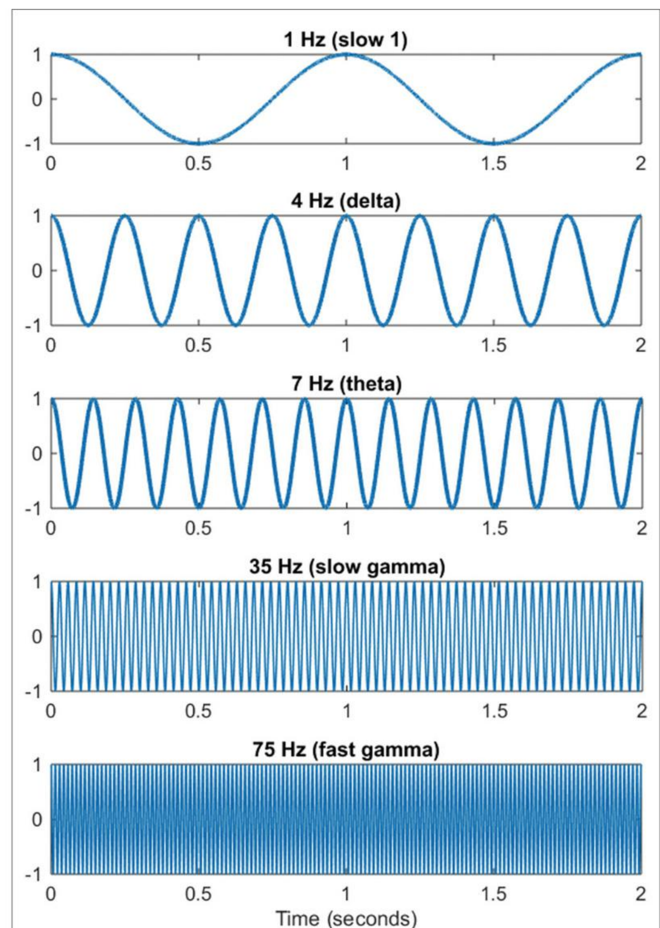
FIGURE 2 | Oscillations of varying frequency. MATLAB generated sine curves to represent neuronal oscillations that make up the unfiltered electroencephalogram (EEG). Each panel represents a distinct frequency and in parentheses the corresponding oscillatory band name most often associated with it.
